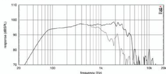
FREQUENCY RESPONSE MADE IN 1/2" L.T. ENCLOSURE TUNED AT 50 Hz IN FREE FIELD (841) ENVIRONMENT. ENCLOSURE CLOSES THE REAR OF THE DRIVER, THE THIN LINE REPRESENTS 45° OFF AXIS FREQUENCY RESPONSE.
